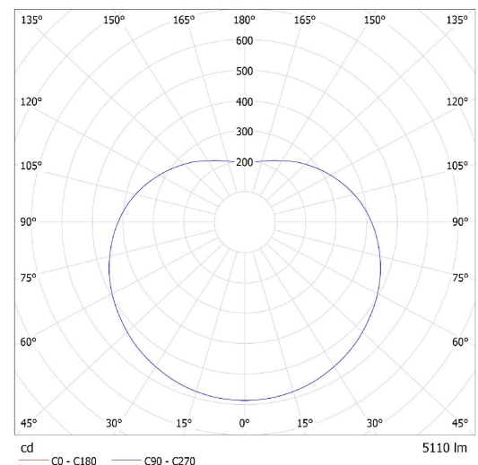
Lucis ZK.P3.400.X POLARIS ZK LED / LDC (Polar)
